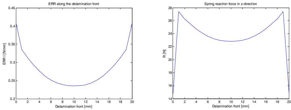
Fig. 6. ERR I and spring reaction force in z-direction along the delamination front
