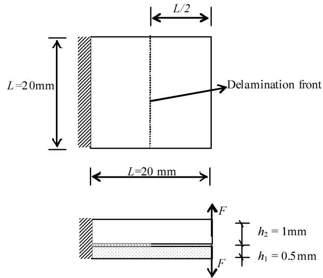
Fig. 3. Laminates geometry
