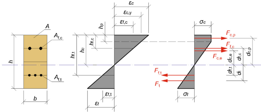
Fig. 1. The adopted assumptions of the analytical model in cross section
