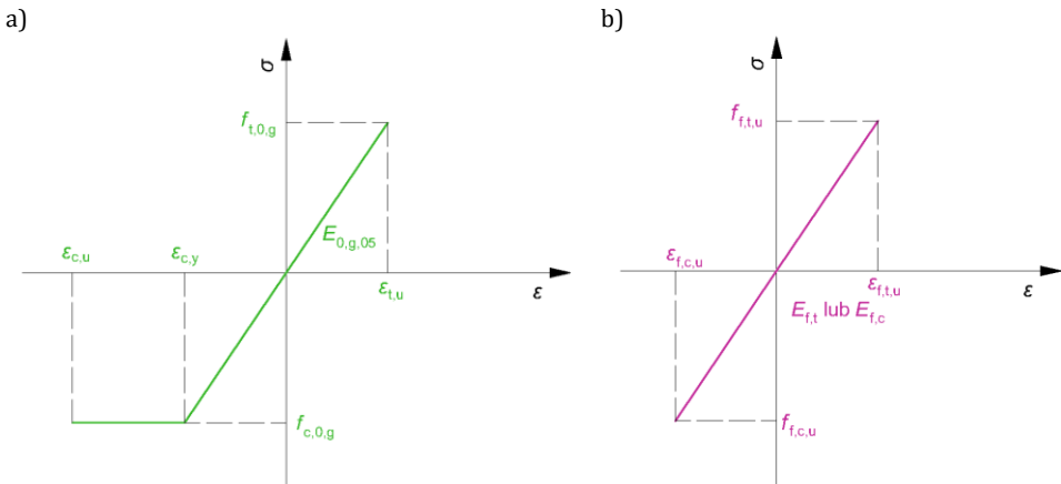
Fig. 2. Material models used for analytical calculations: a) glulam, b) BFRP bars
